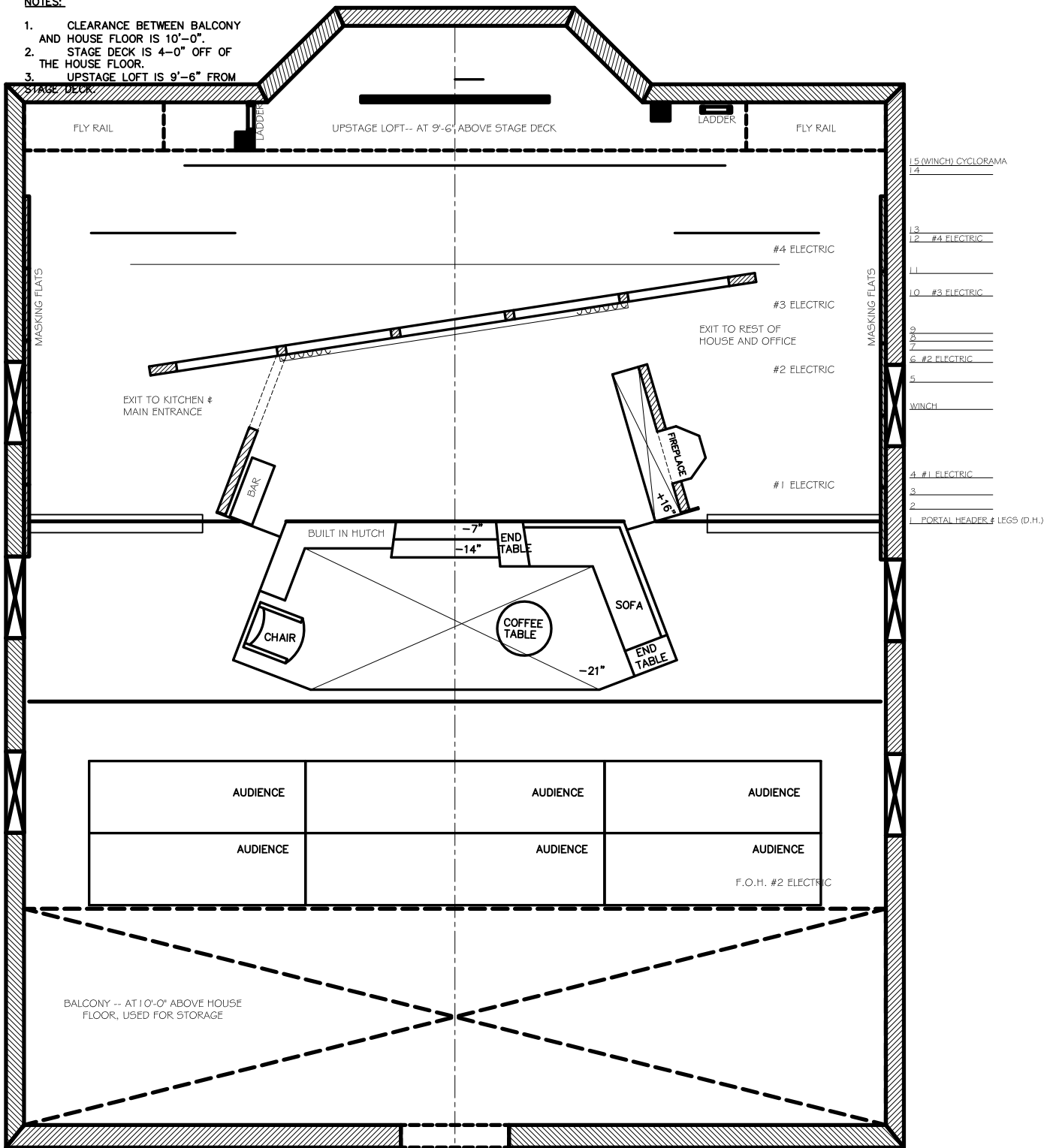
1/8" GROUNDPLAN
